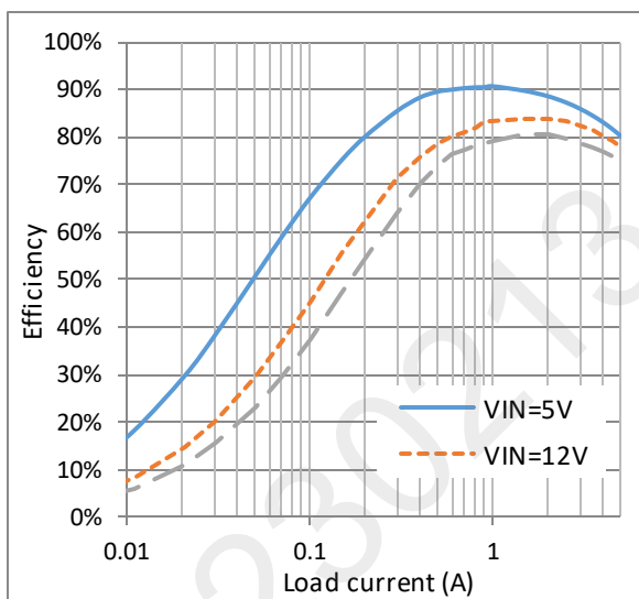
Figure 9. Efficiency vs Load Current ( V_{OUT}=1V , L=1\mu H )
