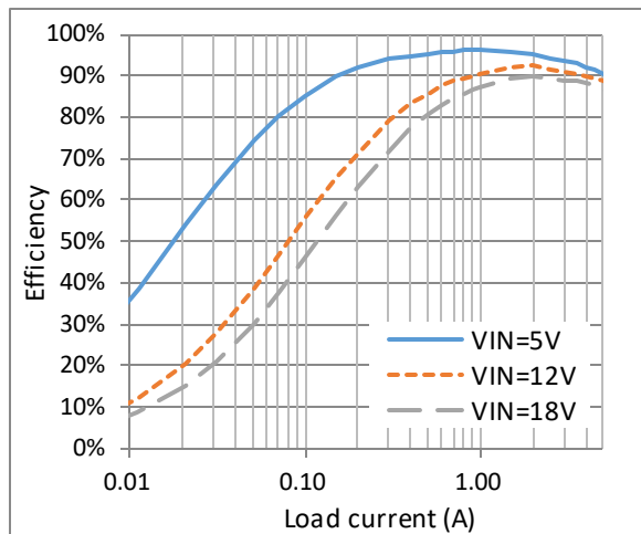
Figure 7. Efficiency vs Load Current ( V_{OUT}=3.3V , L=2.2\mu H )
