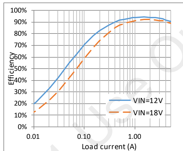
Figure 8. Efficiency vs Load Current ( V_{OUT}=5V , L=3.3\mu H )
