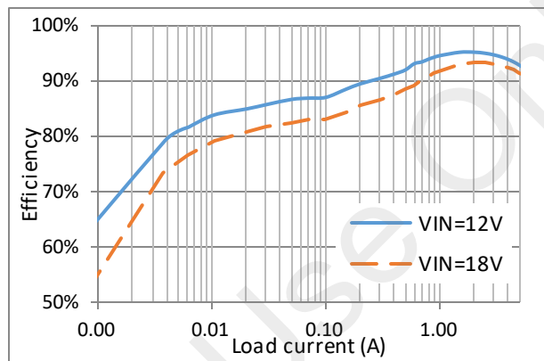
Figure 2. Efficiency vs IOUT (VOUT=5V, L=3.3uH)
