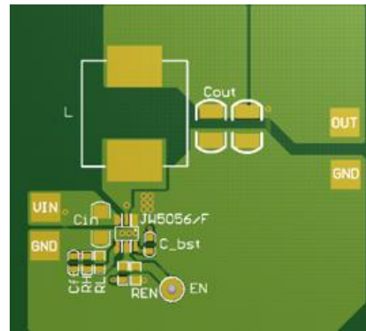
Figure 10. JW5056/F_TSOT23-6 PCB Layout Recommendation
